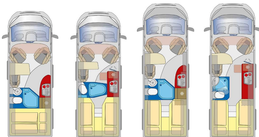
SUMMIT SHINE 600 R
